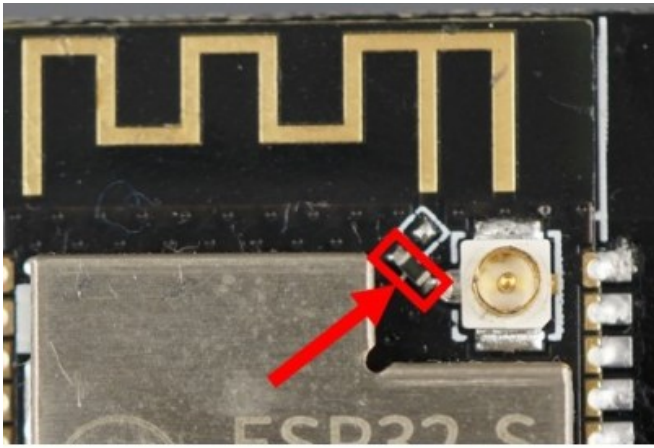
External Antenna
