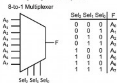
Fig. 6.7 8-to-1 Multiplexer Functionality
