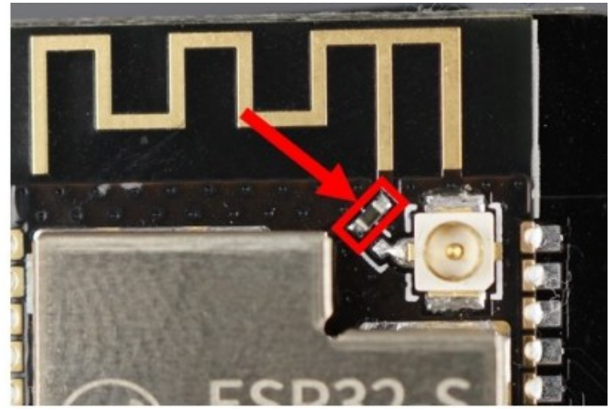
On-board Antenna
