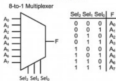
Fig. 6.7 8-to-1 Multiplexer Functionality
