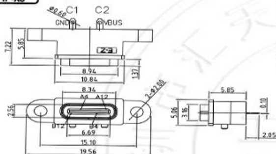
PIN ASSIGNMENT
